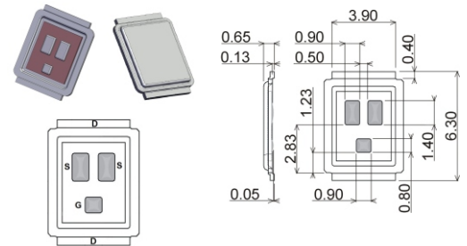
DirectFET
