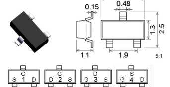
SOT23 / TO236AB
