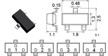
SOT23 / TO236AB
