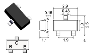
SOT23 / TO236AB
