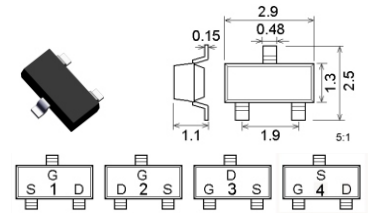
SOT23 / TO236AB
