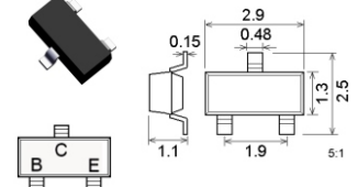
SOT23 / TO236AB
