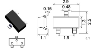
SOT23 / TO236AB
