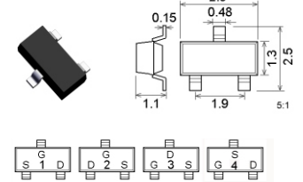
SOT23 / TO236AB
