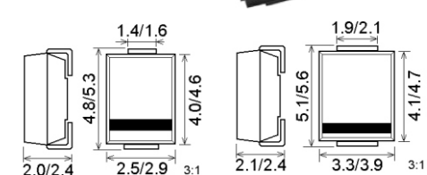
SMC (DO214AB)
